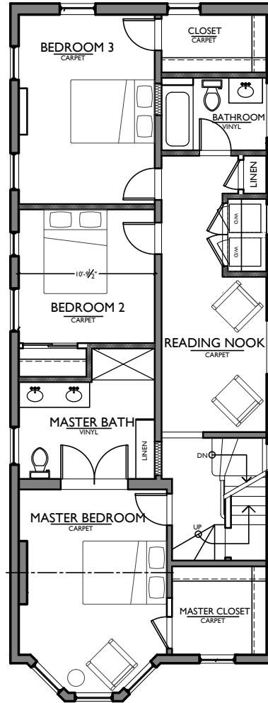
Second Floor
